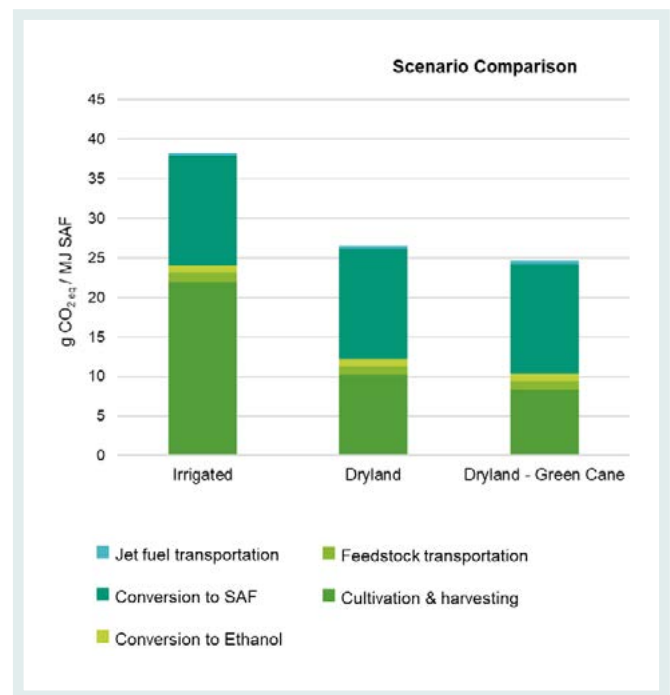
Lifecycle GHG emissions for SAF produced from South African irrigated and dryland sugarcane
